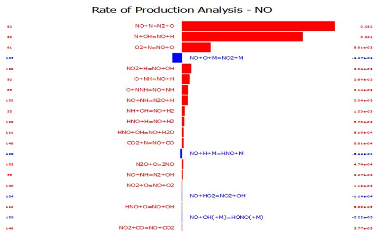
Figure 3.4: Adiabatic batch reactor: rate of production analyses for H2O and NO as calculated by using the OpenSMOKE++ PostProcessor.
